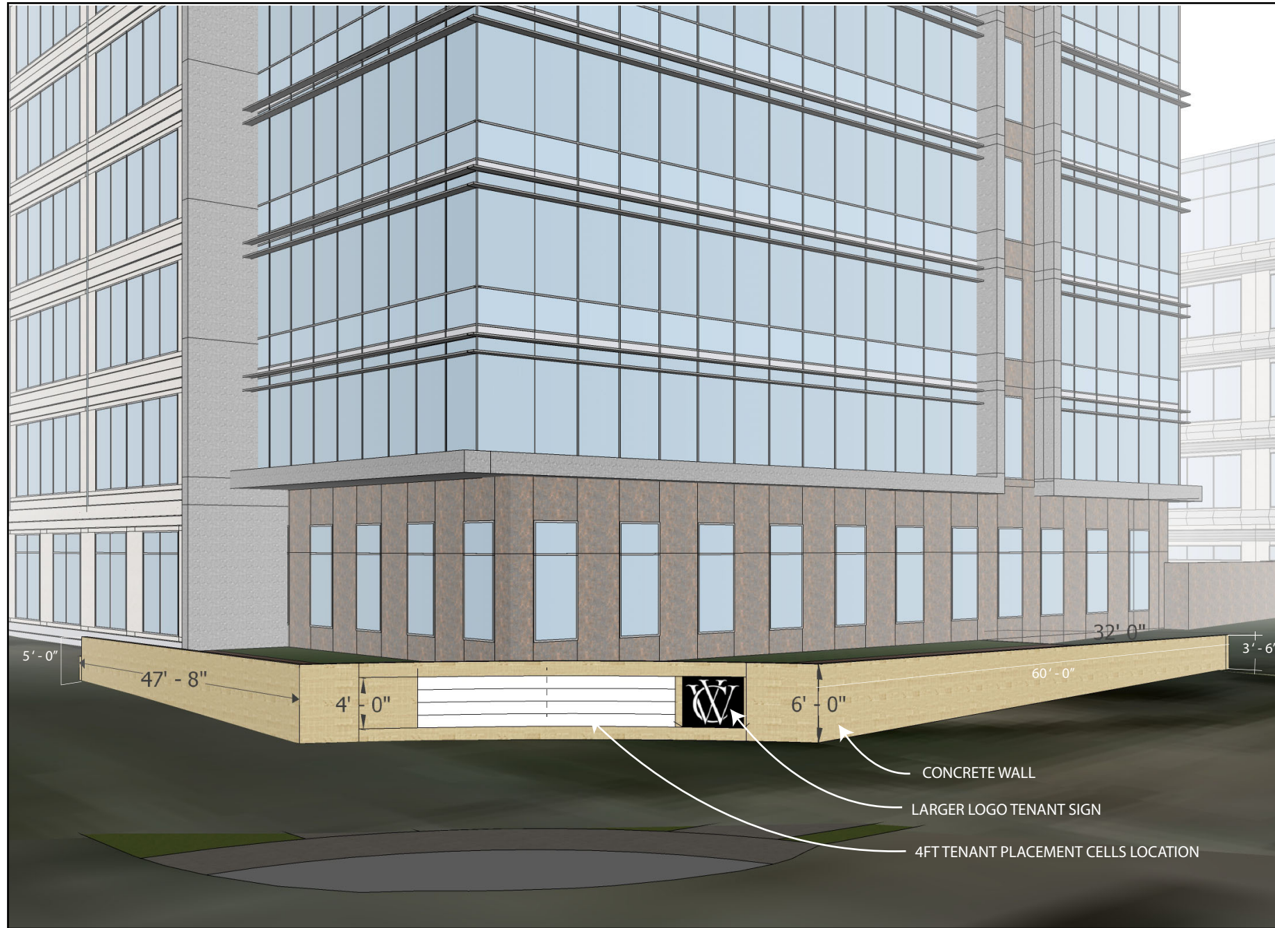
PERSPECTIVE VIEW
