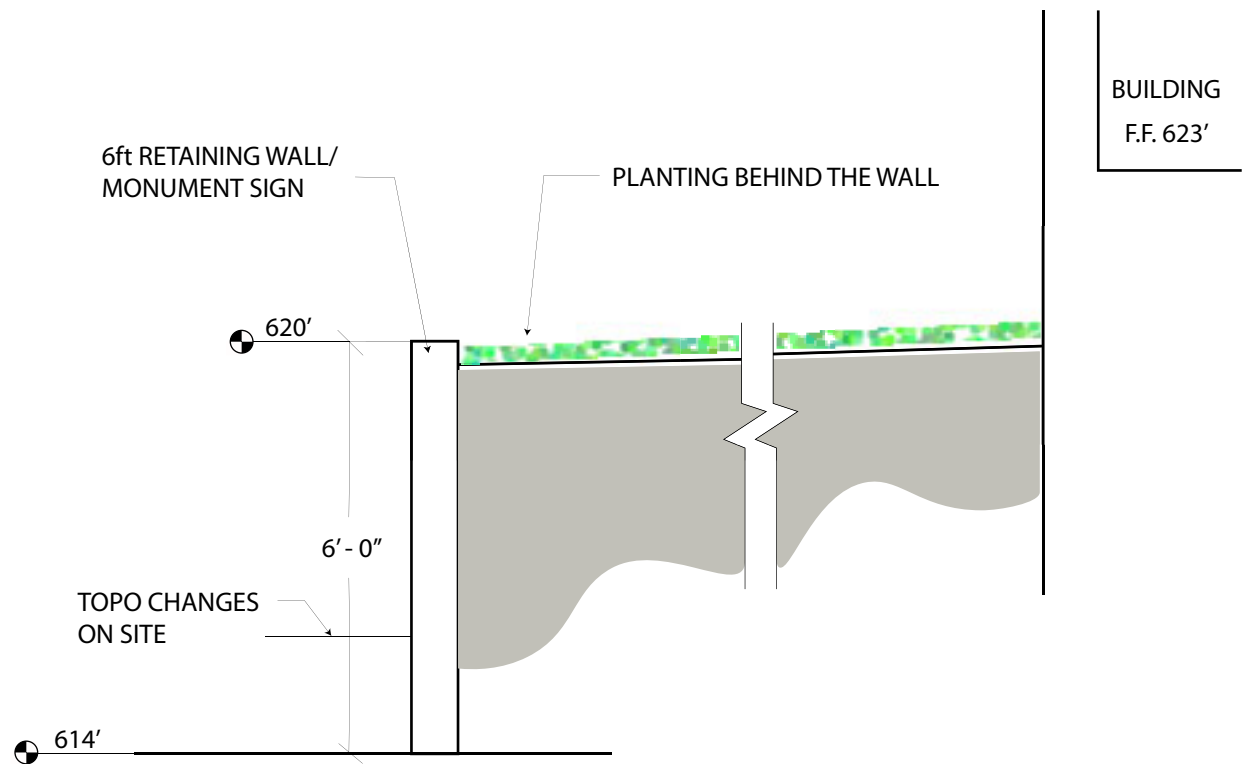
SECTION DIAGRAM
